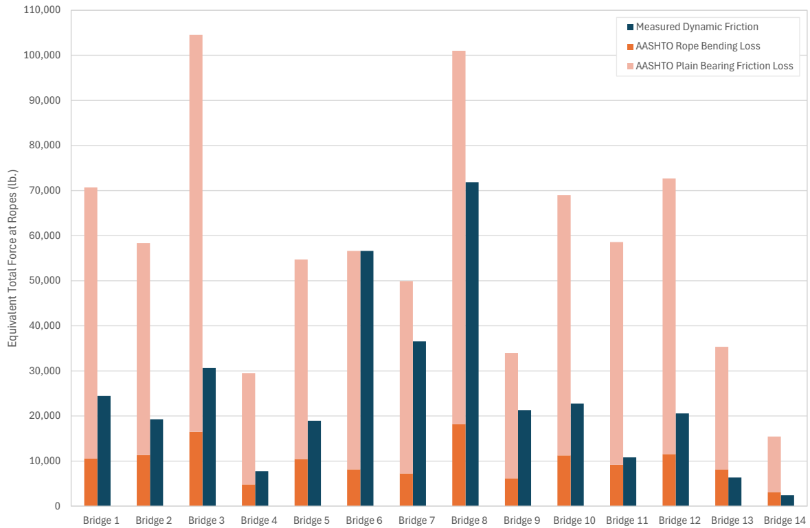
Vertical Lift Bridges w/ Plain Trunnion Bearings AASHTO Dynamic Friction Versus Measured
